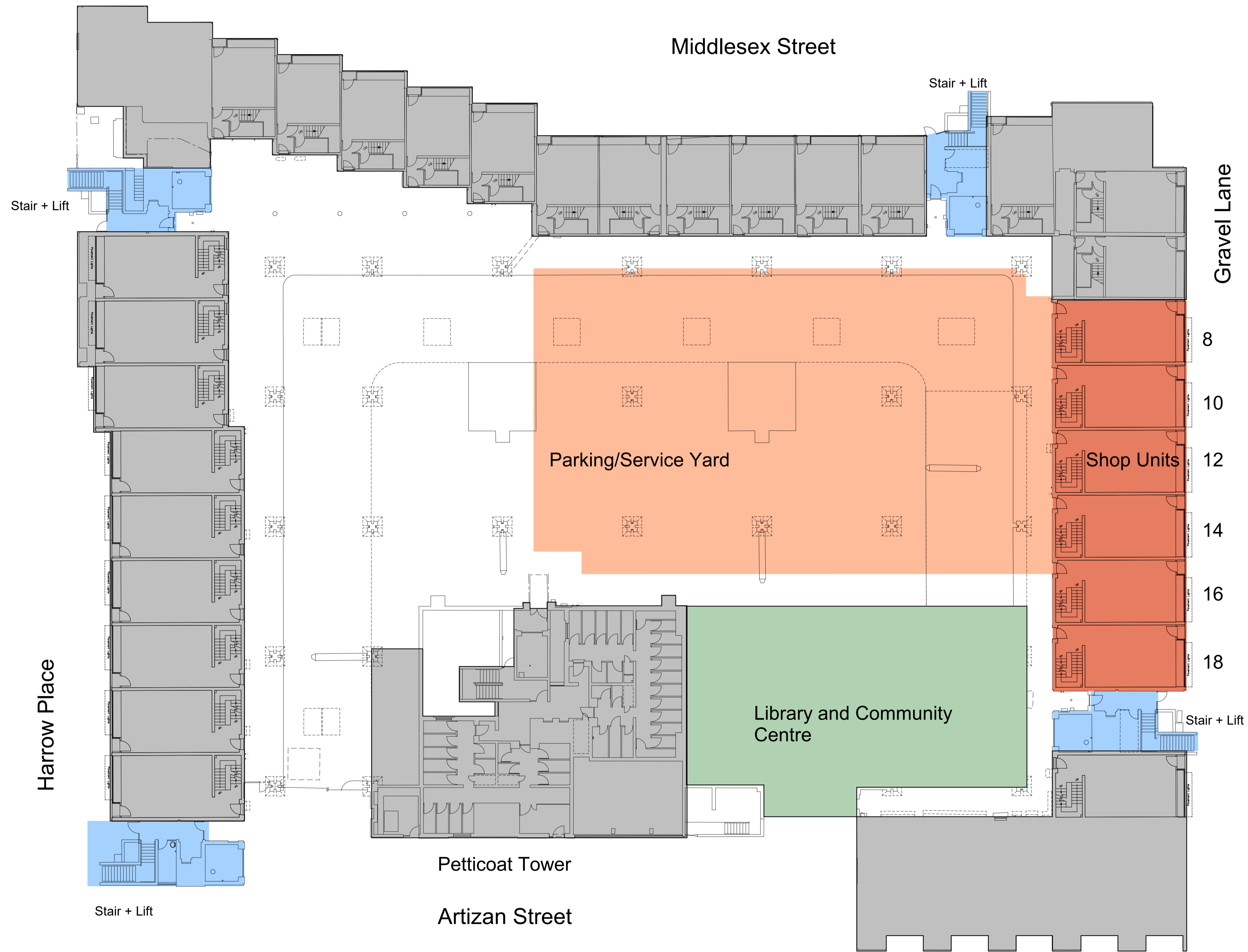
Ground Floor - Key Plan 1 : 200
